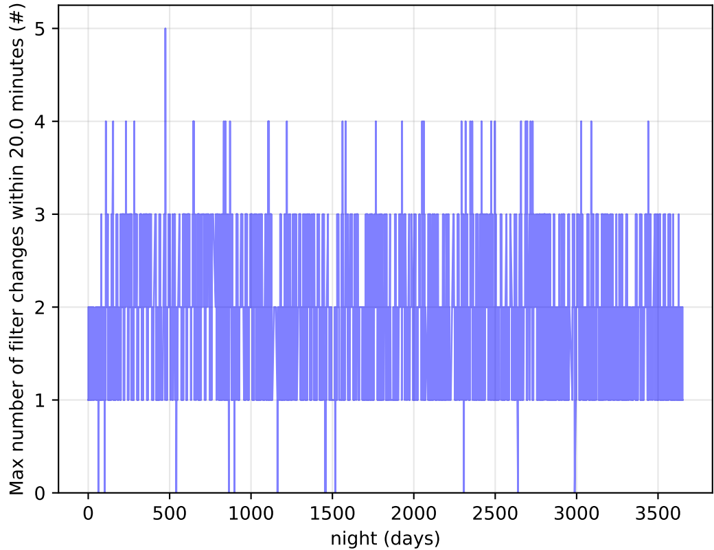
internal_u_expt27_nscale1.2v3.4_10yrs Per Night: Max number of filter changes within 20.0 minutes
