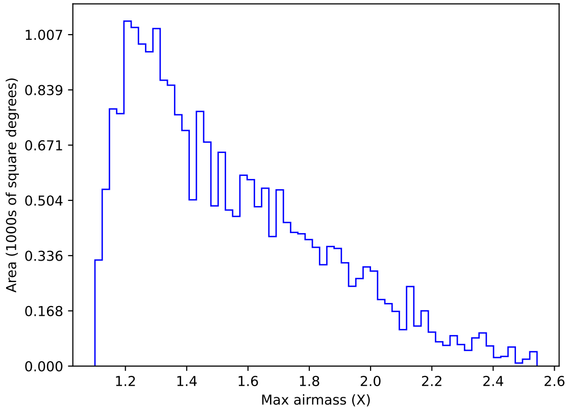
internal_u_expt27_nscale1.2v3.4_10yrs Yr 1 u band: Max airmass
