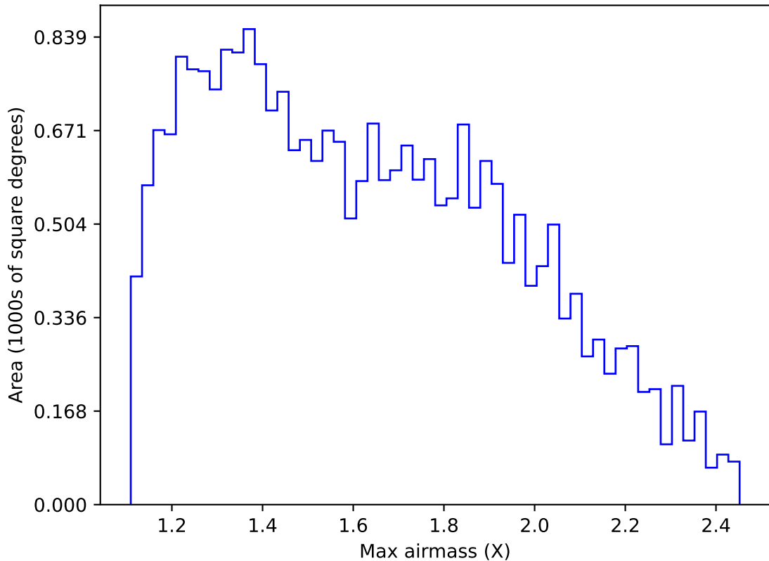
internal_u_expt27_nscale1.2v3.4_10yrs Yr 1 g band: Max airmass
