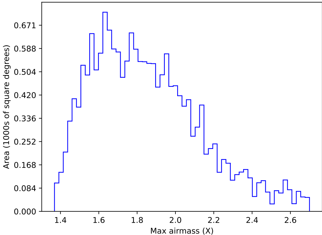
internal_u_expt27_nscale1.2v3.4_10yrs WFD u band: Max airmass
