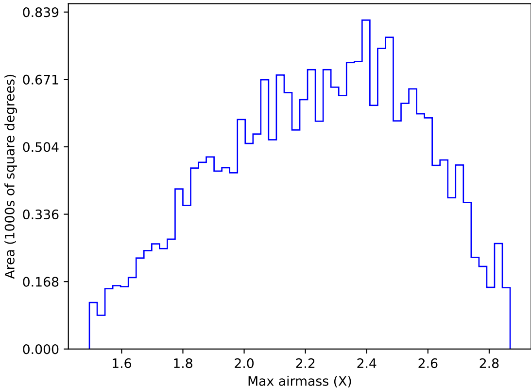
internal_u_expt27_nscale1.2v3.4_10yrs All sky y band: Max airmass
