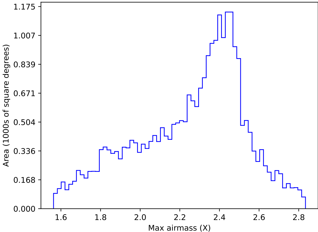
internal_u_expt27_nscale1.2v3.4_10yrs All sky r band: Max airmass
