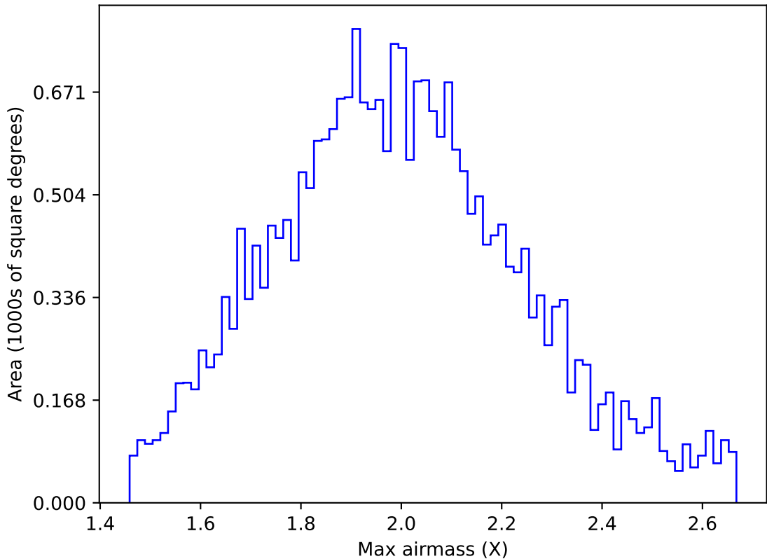
internal_u_expt27_nscale1.2v3.4_10yrs All sky g band: Max airmass
