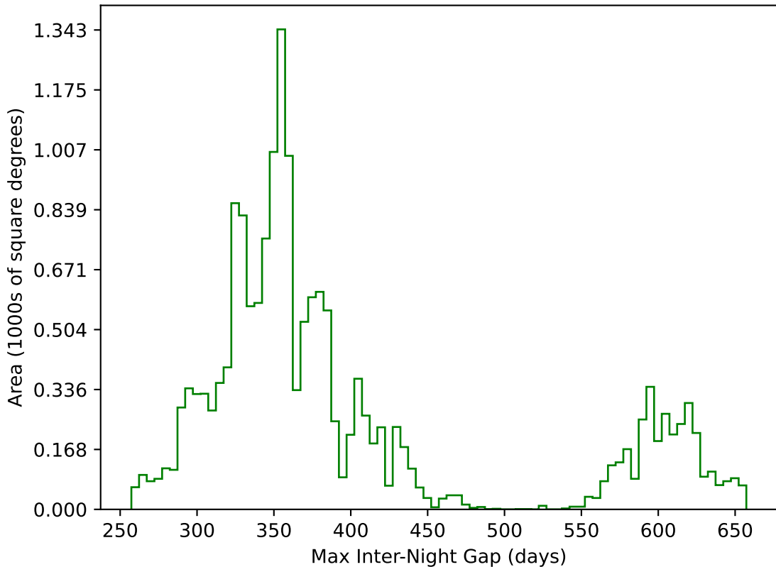
internal_u_expt27_nscale1.2v3.4_10yrs WFD g band: Max Inter-Night Gap
