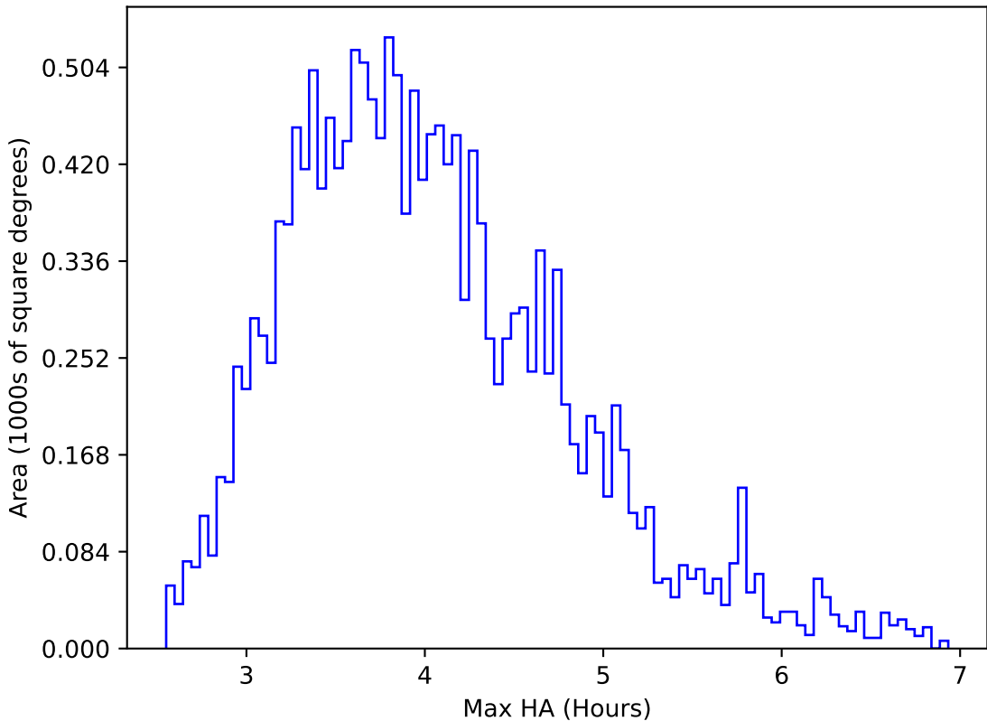
internal_u_expt27_nscale1.2v3.4_10yrs WFD g band: Max HA
