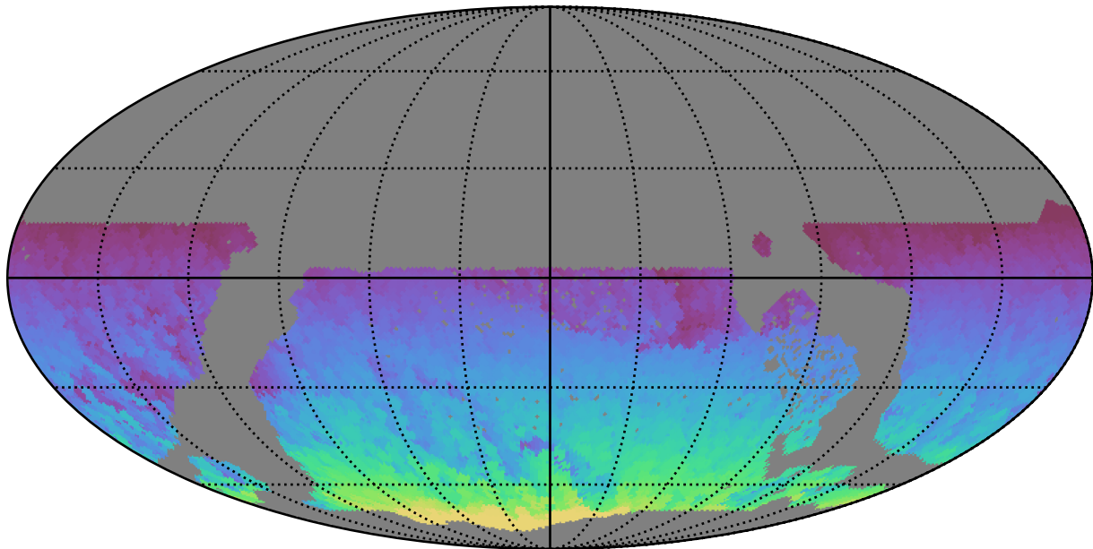
internal_u_expt27_nscale1.2v3.4_10yrs WFD all bands: Max HA
