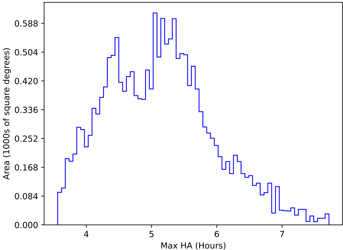
internal_u_expt27_nscale1.2v3.4_10yrs WFD all bands: Max HA
