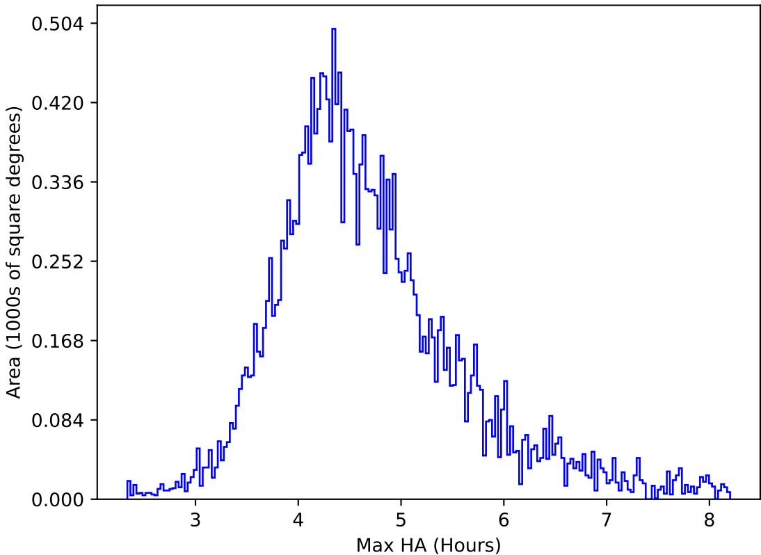
internal_u_expt27_nscale1.2v3.4_10yrs All sky y band: Max HA
