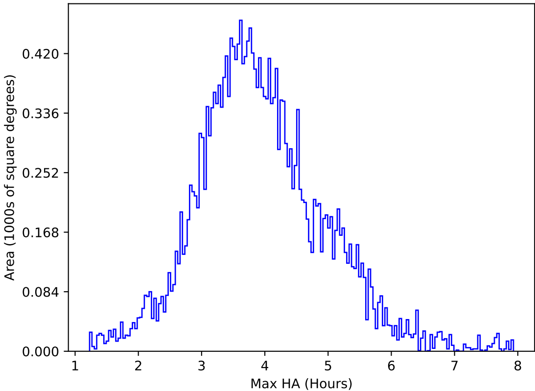
internal_u_expt27_nscale1.2v3.4_10yrs All sky u band: Max HA
