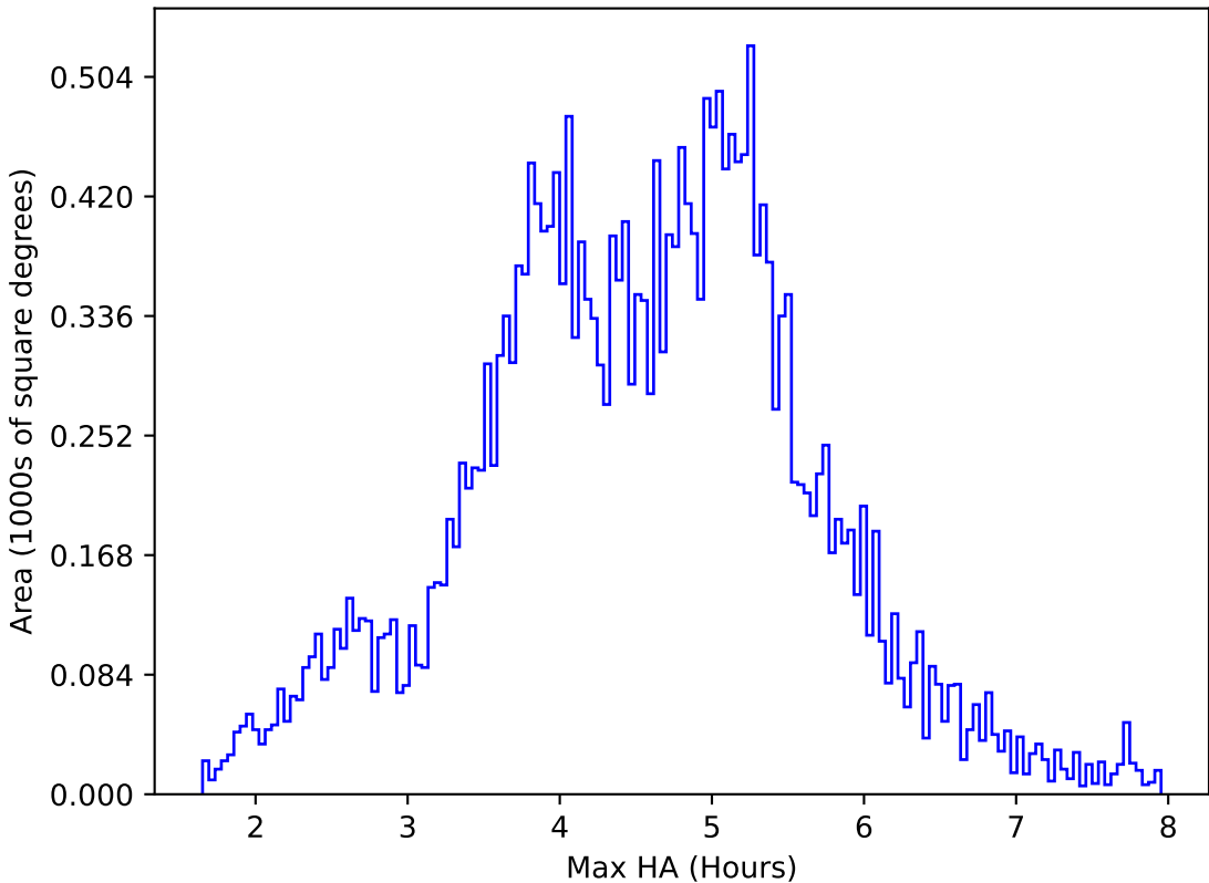
internal_u_expt27_nscale1.2v3.4_10yrs All sky i band: Max HA
