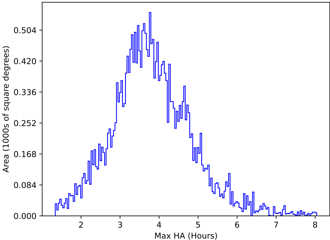
internal_u_expt27_nscale1.2v3.4_10yrs All sky g band: Max HA
