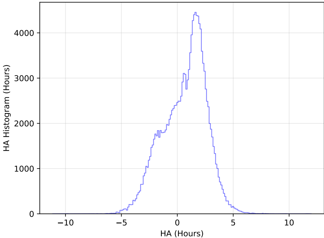
internal_u_expt27_nscale1.2v3.4_10yrs WFD u band: HA Histogram
