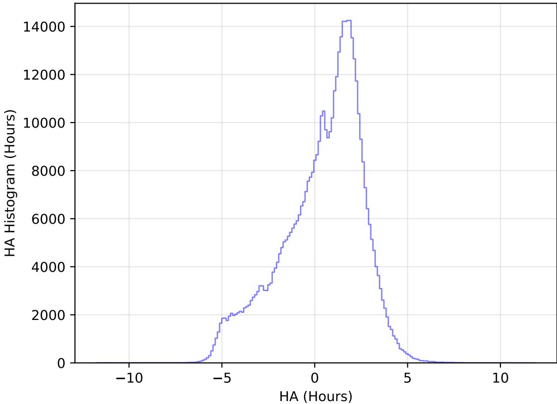
internal_u_expt27_nscale1.2v3.4_10yrs WFD r band: HA Histogram
