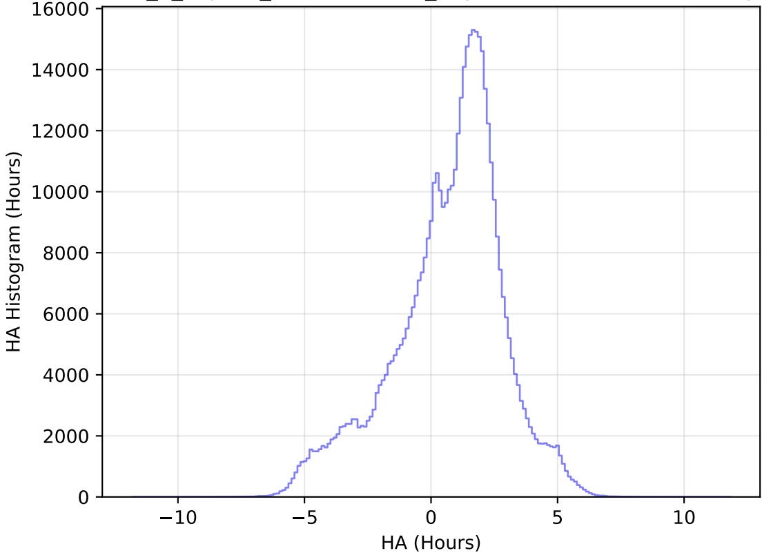
internal_u_expt27_nscale1.2v3.4_10yrs WFD i band: HA Histogram
