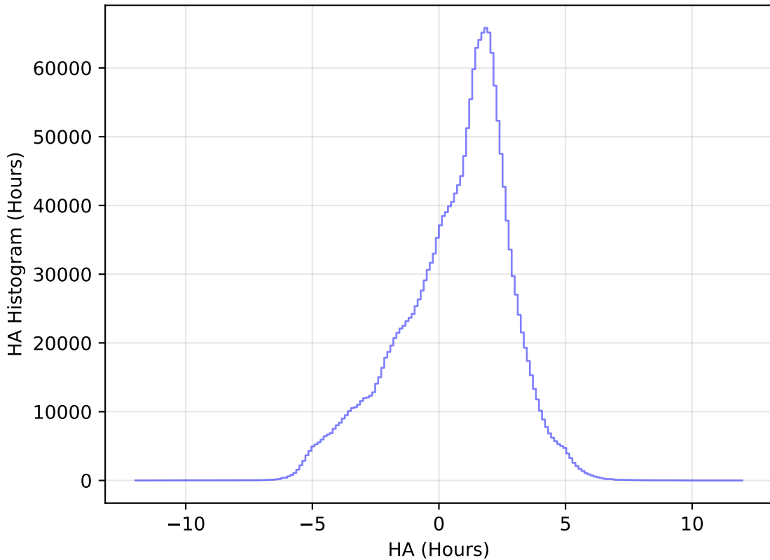
internal_u_expt27_nscale1.2v3.4_10yrs WFD all bands: HA Histogram
