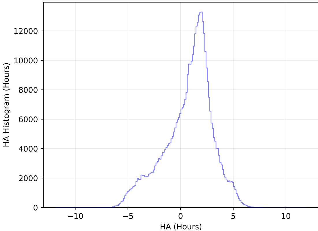
internal_u_expt27_nscale1.2v3.4_10yrs All sky z band: HA Histogram
