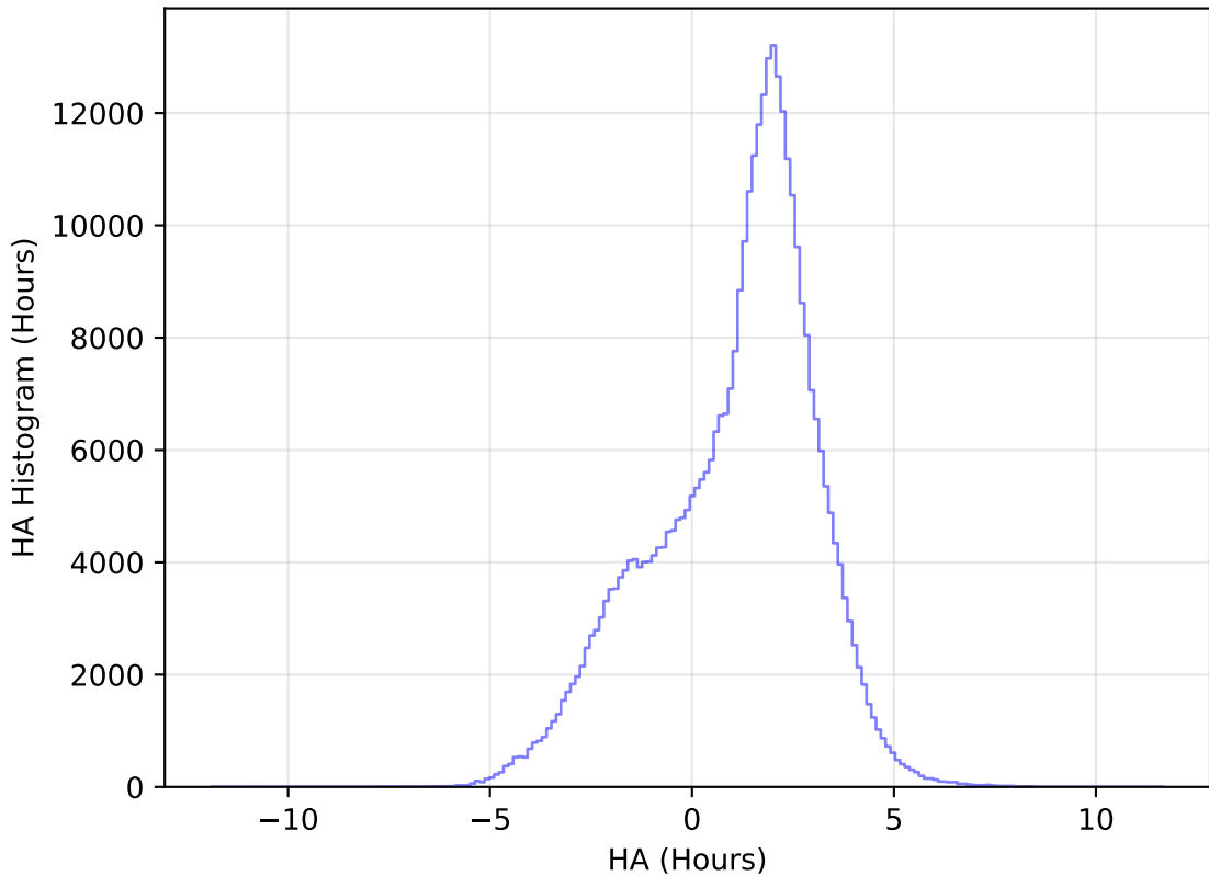
internal_u_expt27_nscale1.2v3.4_10yrs All sky y band: HA Histogram
