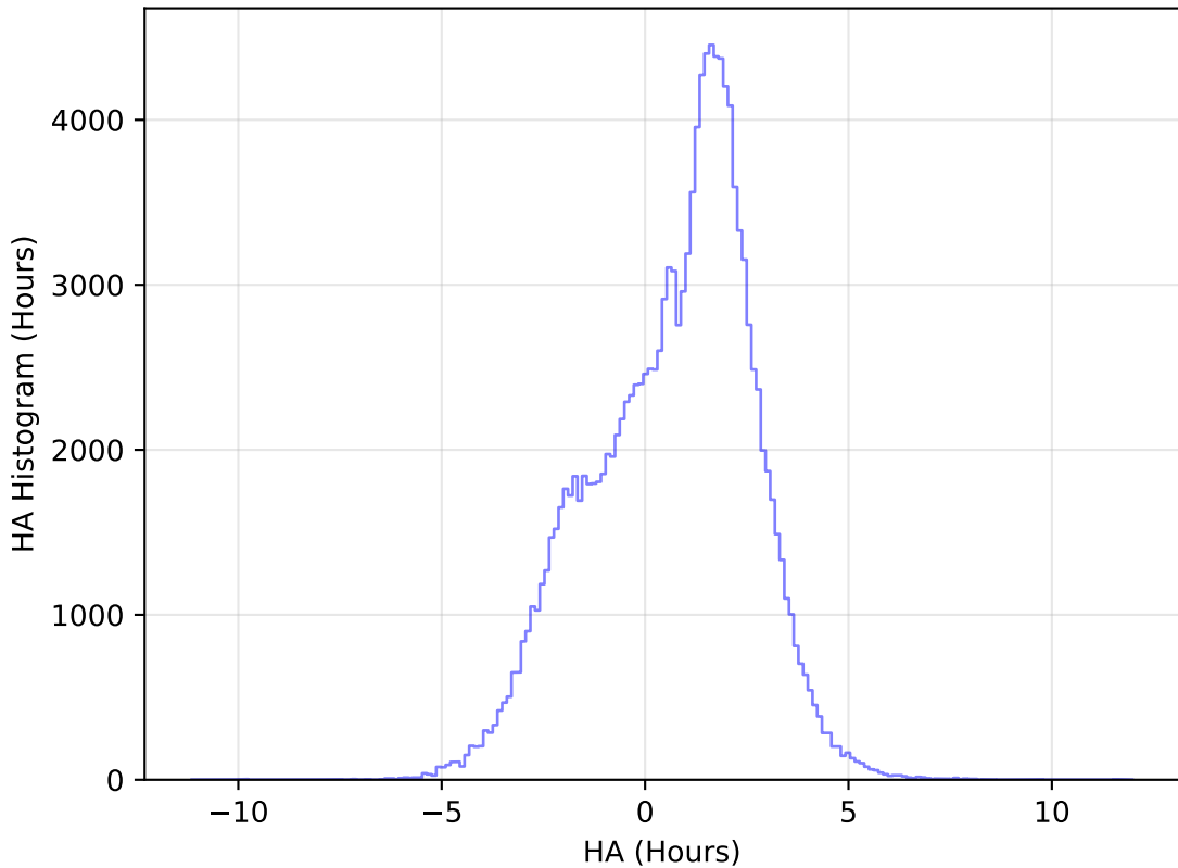
internal_u_expt27_nscale1.2v3.4_10yrs All sky u band: HA Histogram
