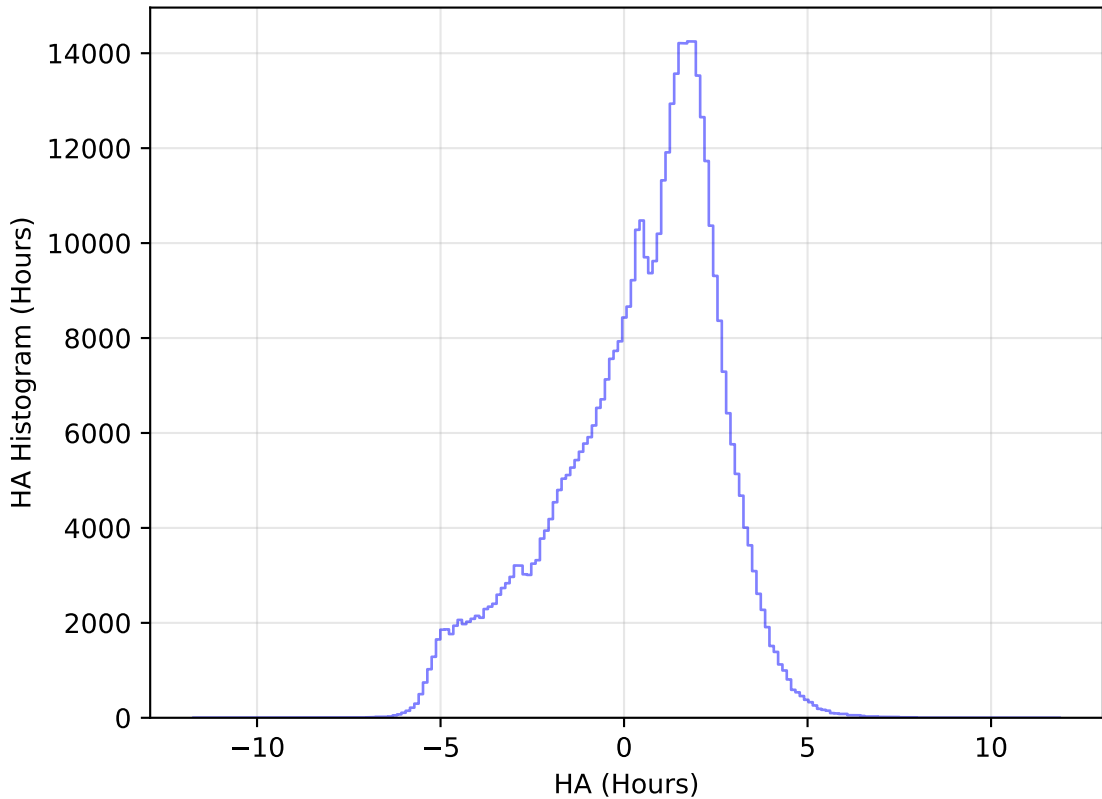
internal_u_expt27_nscale1.2v3.4_10yrs All sky r band: HA Histogram
