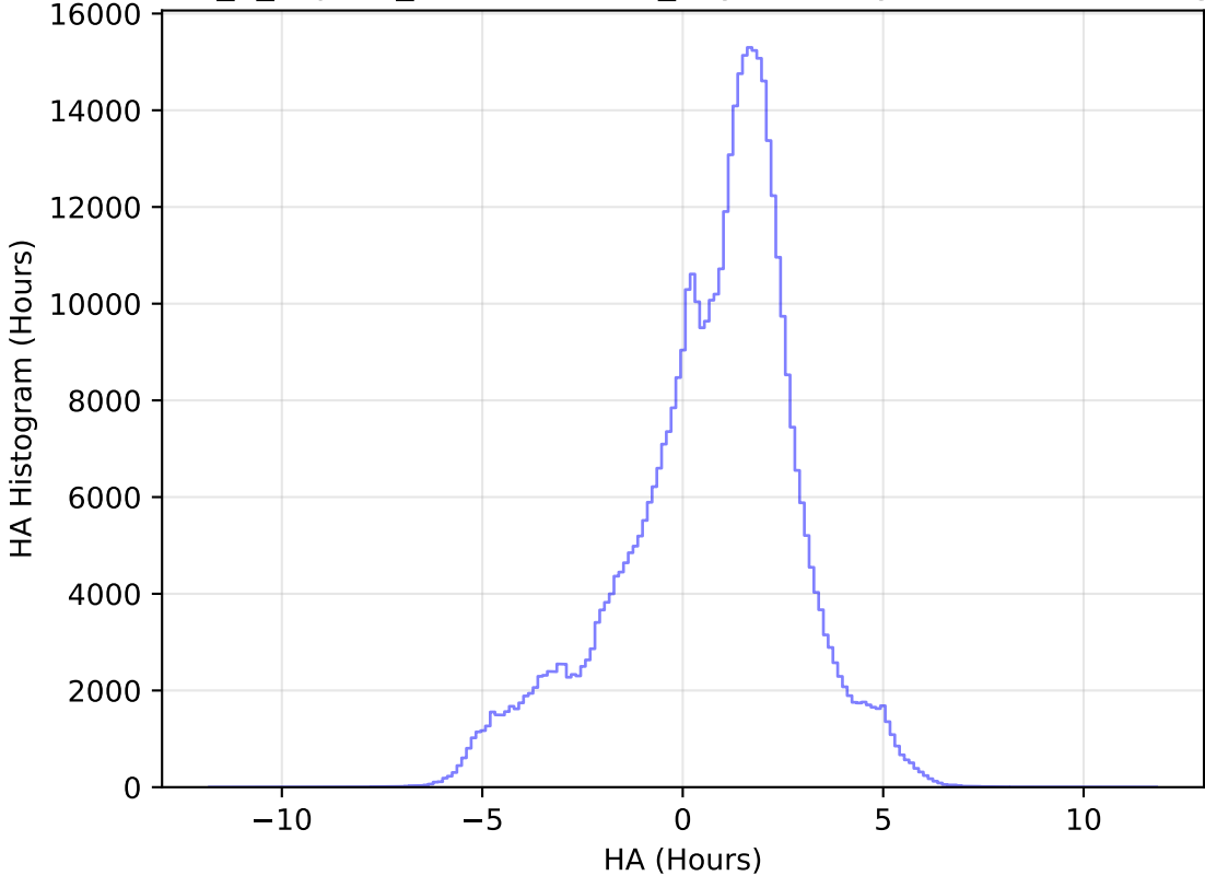
internal_u_expt27_nscale1.2v3.4_10yrs All sky i band: HA Histogram
