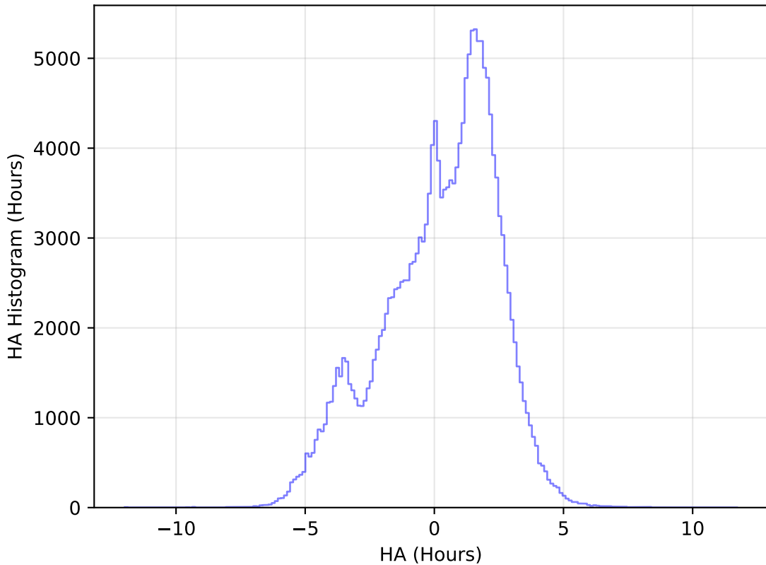
internal_u_expt27_nscale1.2v3.4_10yrs All sky g band: HA Histogram
