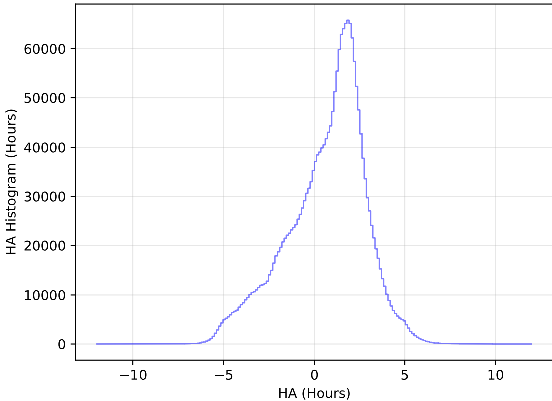
internal_u_expt27_nscale1.2v3.4_10yrs All sky all bands: HA Histogram
