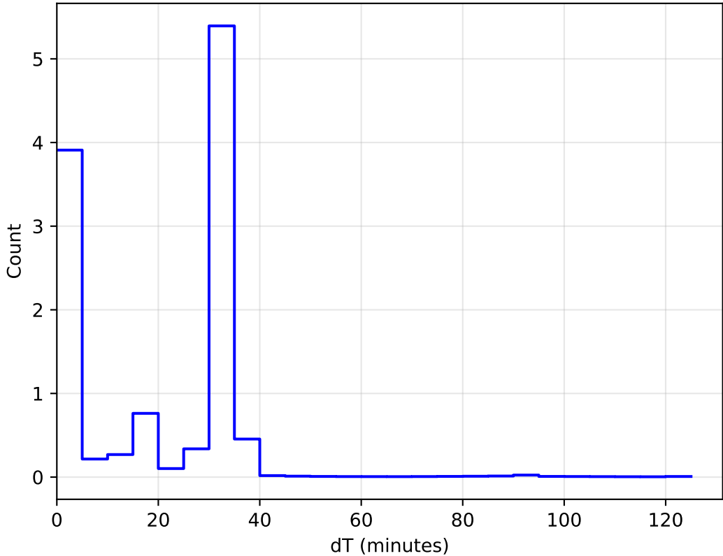
internal_u_expt27_nscale1.2v3.4_10yrs WFD: DeltaT Histogram
