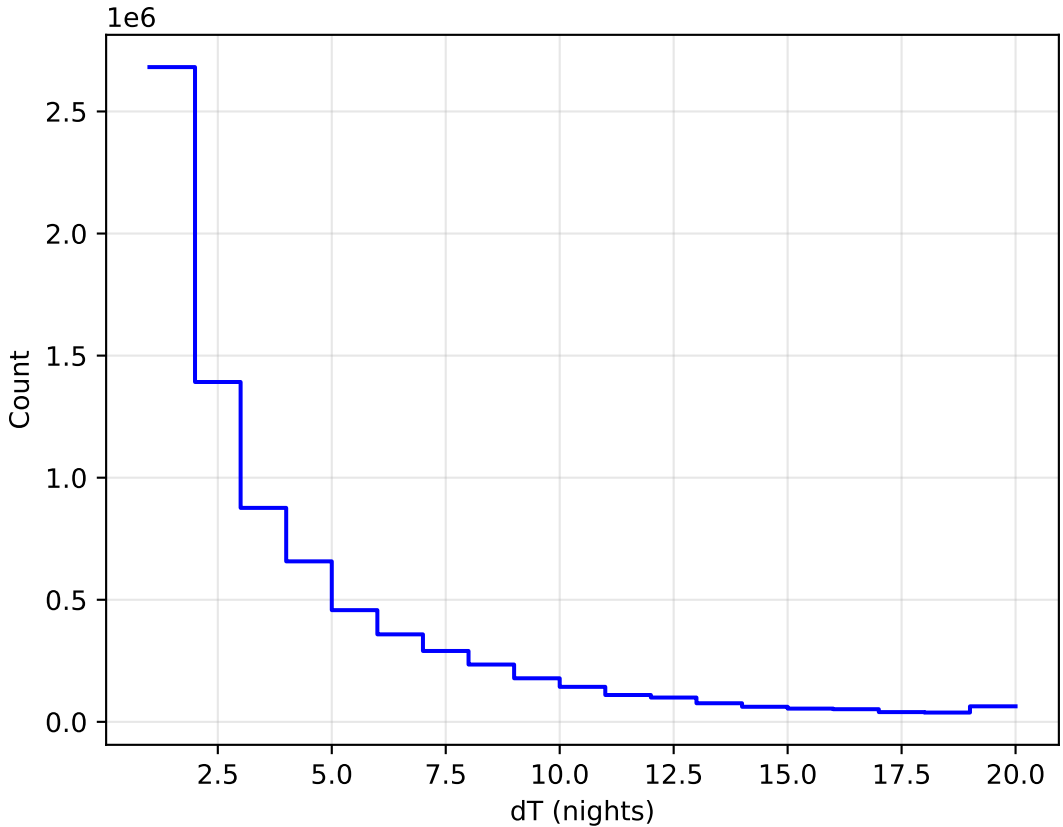
internal_u_expt27_nscale1.2v3.4_10yrs WFD all bands: DeltaNight Histogram
