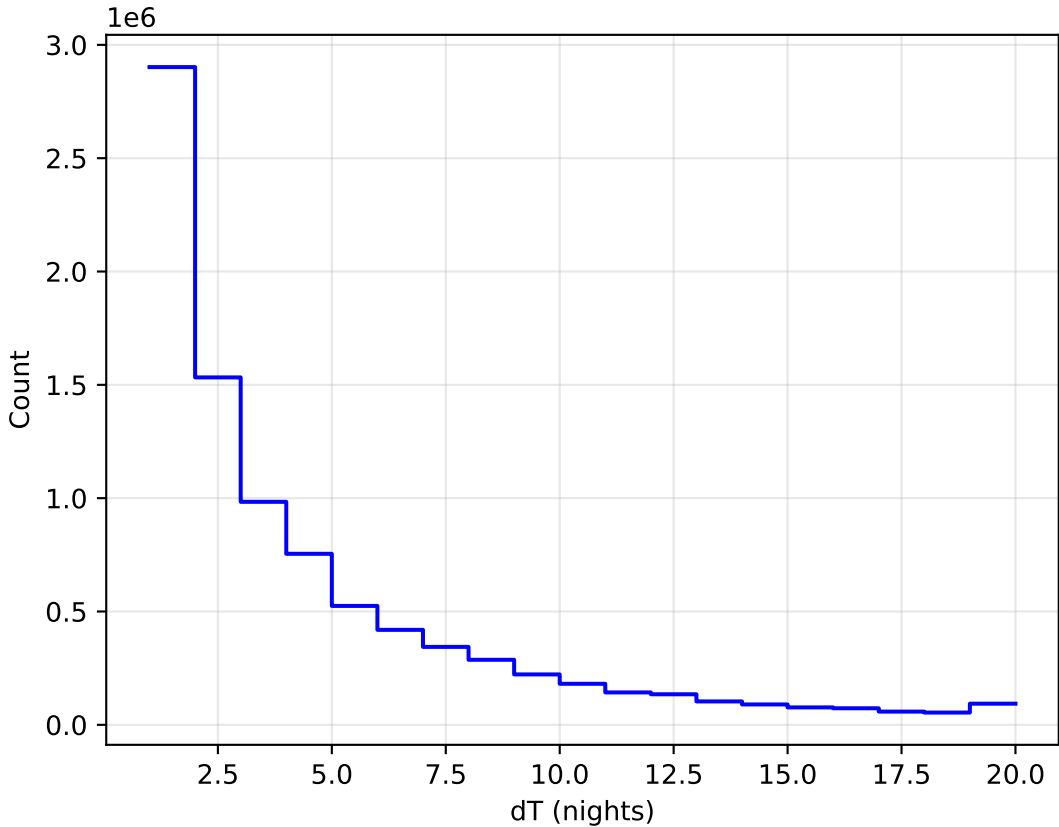
internal_u_expt27_nscale1.2v3.4_10yrs All sky all bands: DeltaNight Histogram
