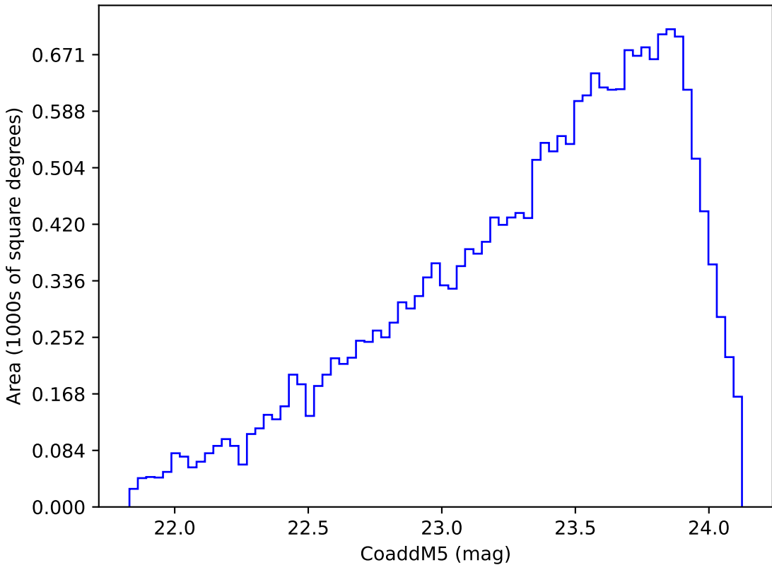
internal_u_expt27_nscale1.2v3.4_10yrs Yr 3-4 y band: CoaddM5
