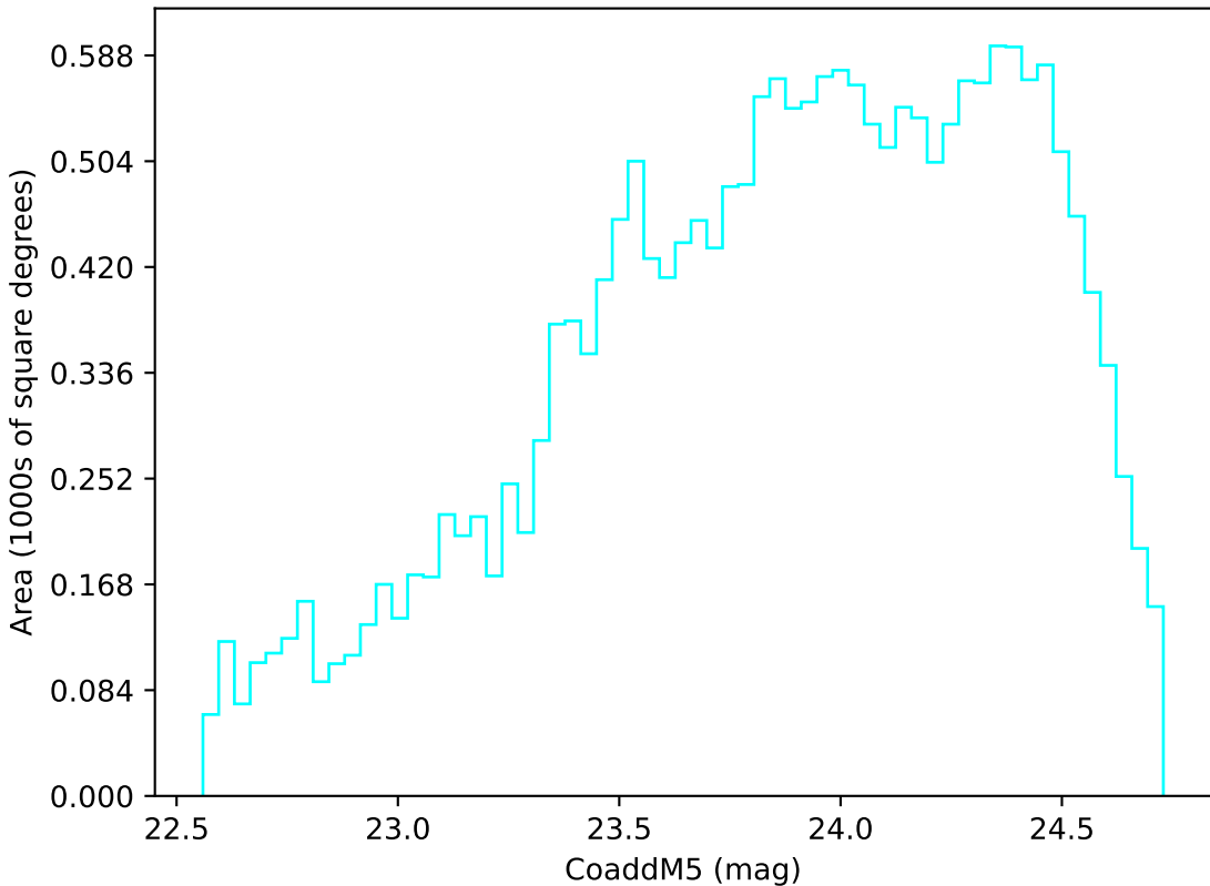
internal_u_expt27_nscale1.2v3.4_10yrs Yr 3-4 u band: CoaddM5
