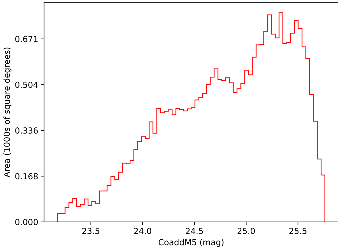
internal_u_expt27_nscale1.2v3.4_10yrs Yr 3-4 i band: CoaddM5
