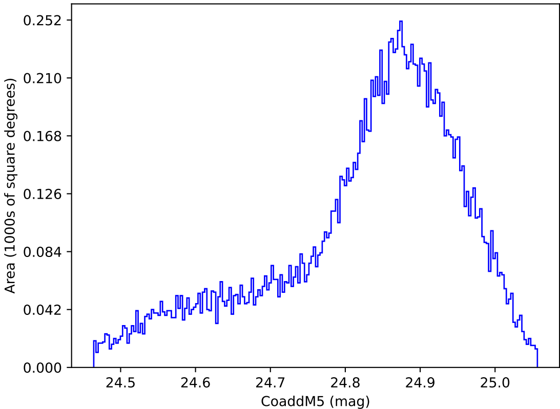
internal_u_expt27_nscale1.2v3.4_10yrs WFD y band: CoaddM5
