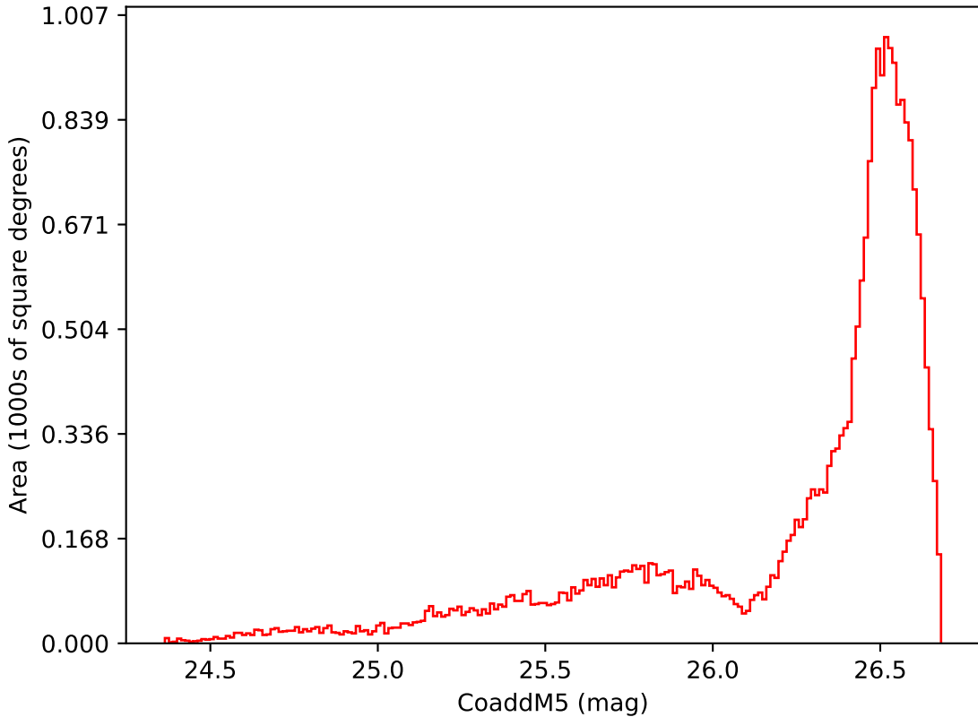
internal_u_expt27_nscale1.2v3.4_10yrs All sky i band: CoaddM5
