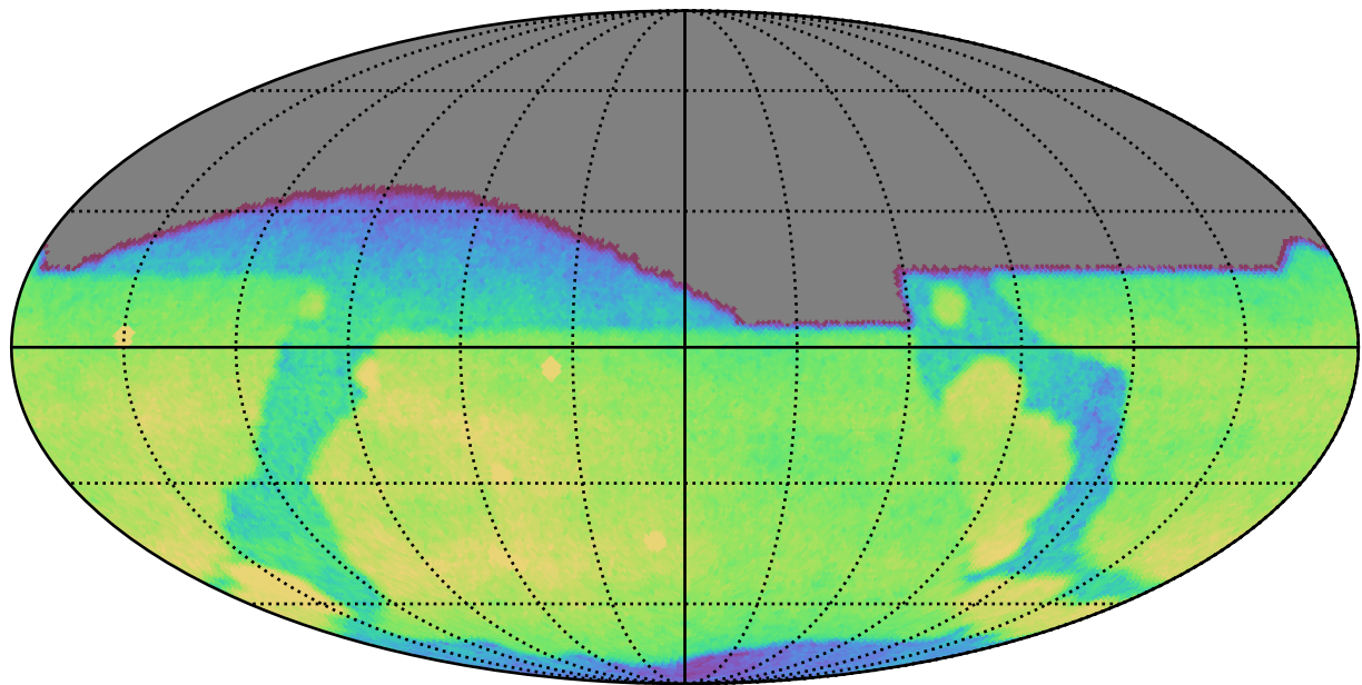
internal_u_expt27_nscale1.2v3.4_10yrs All sky g band: CoaddM5
