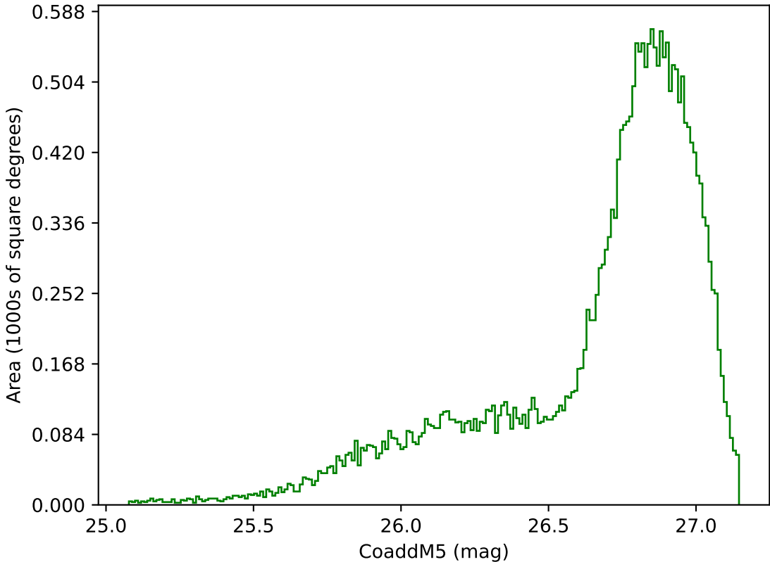
internal_u_expt27_nscale1.2v3.4_10yrs All sky g band: CoaddM5
