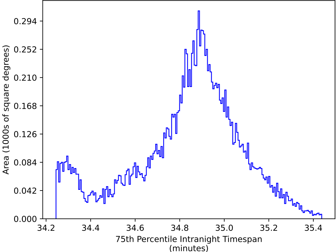
internal_u_expt27_nscale1.2v3.4_10yrs WFD: 75th Percentile Intranight Timespan
