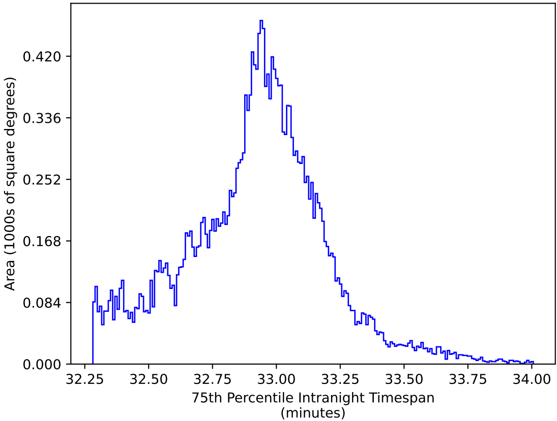
internal_u_expt27_nscale1.2v3.4_10yrs All sky y band: 75th Percentile Intranight Timespan
