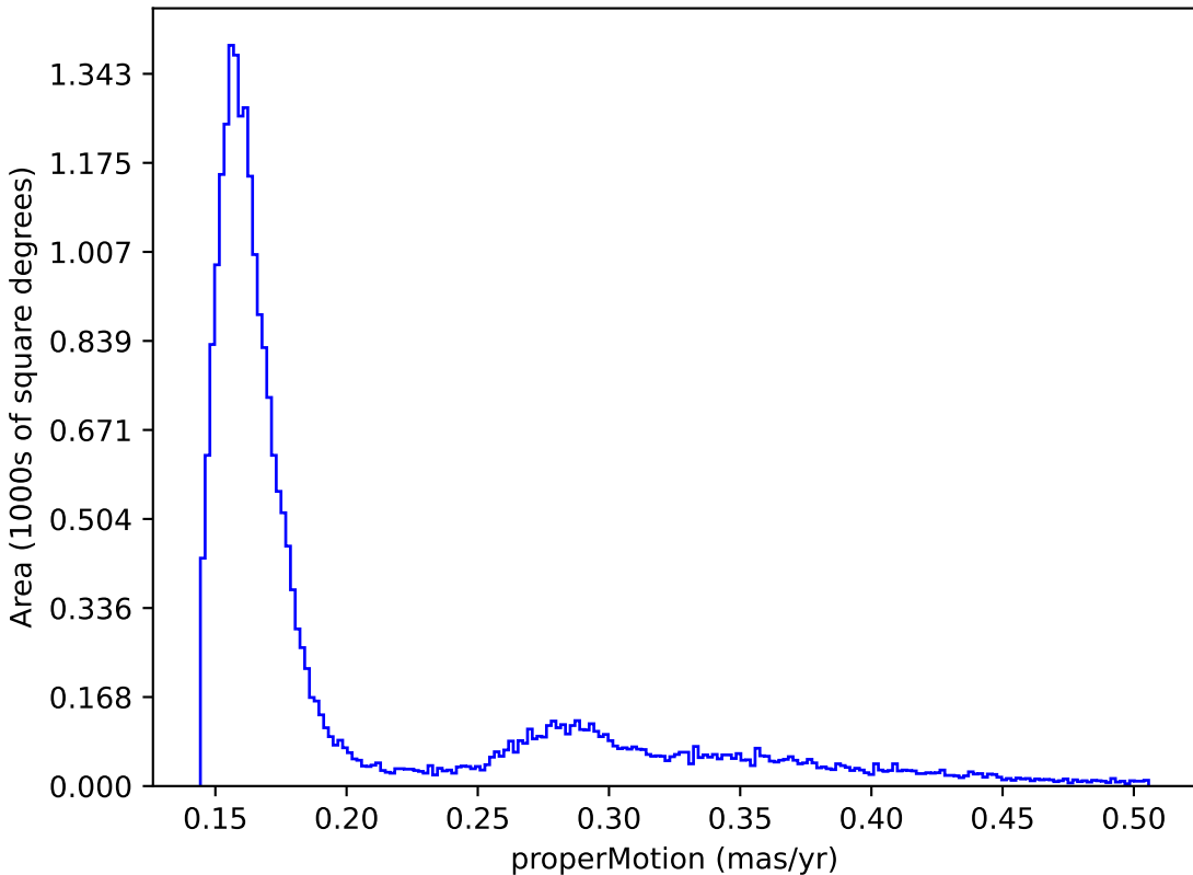
internal_u_expt27_nscale1.2v3.4_10yrs : properMotion
