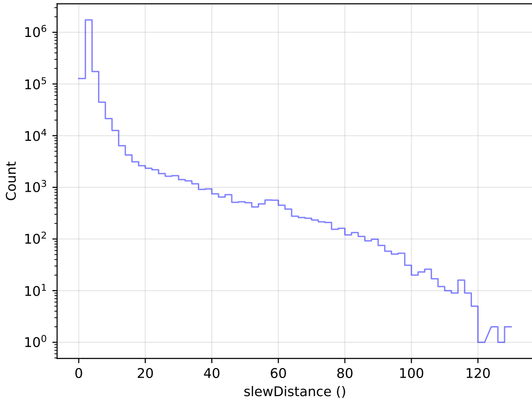
internal_u_expt27_nscale1.2v3.4_10yrs All visits: Slew Distance Histogram
