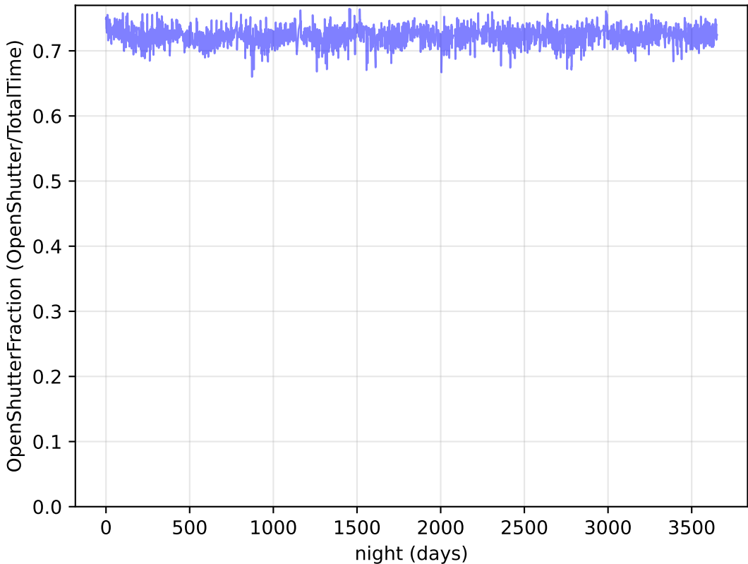
internal_u_expt27_nscale1.2v3.4_10yrs : OpenShutterFraction
