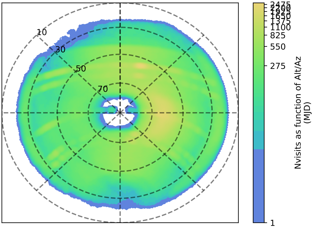
internal_u_expt27_nscale1.2v3.4_10yrs z: Nvisits as function of Alt/Az
