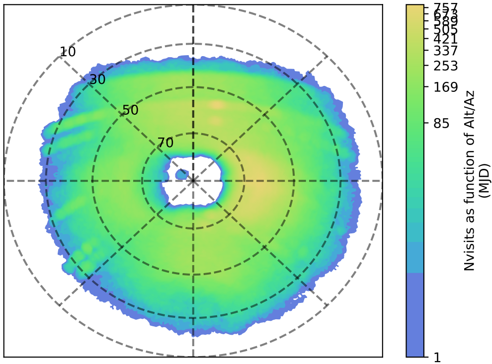
internal_u_expt27_nscale1.2v3.4_10yrs u: Nvisits as function of Alt/Az
