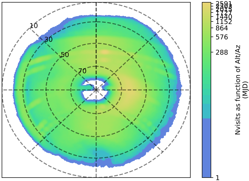
internal_u_expt27_nscale1.2v3.4_10yrs r: Nvisits as function of Alt/Az
