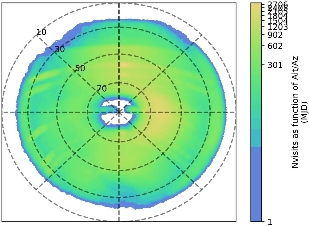
internal_u_expt27_nscale1.2v3.4_10yrs i: Nvisits as function of Alt/Az
