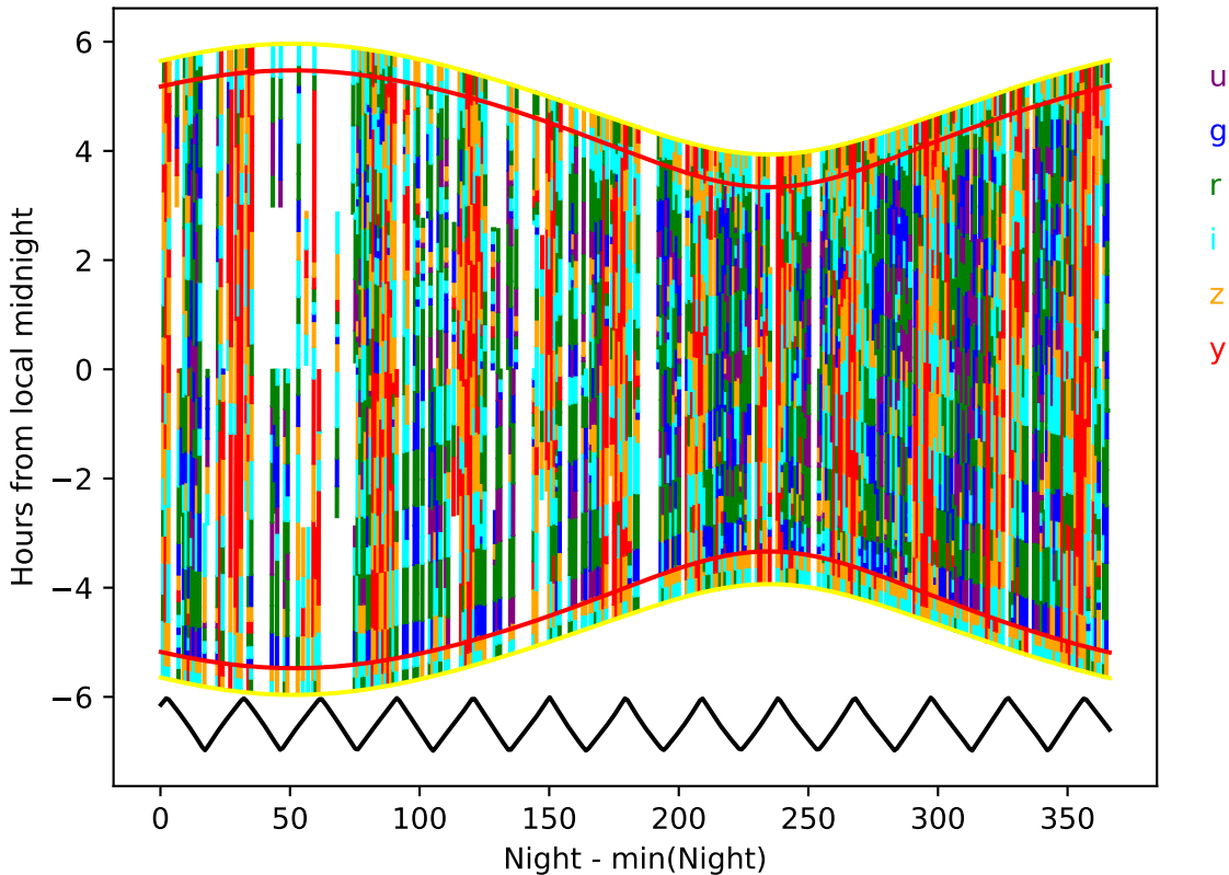
internal_u_expt27_nscale1.2v3.4_10yrs year 9-10: Hourglass
