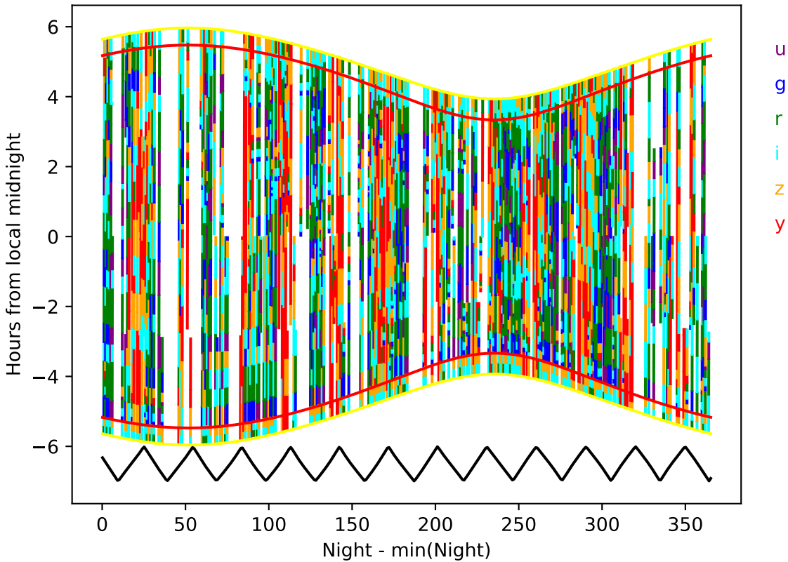
internal_u_expt27_nscale1.2v3.4_10yrs year 7-8: Hourglass
