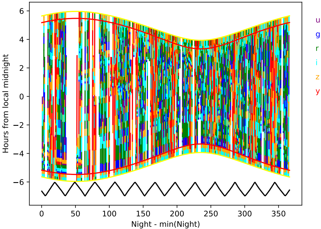
internal_u_expt27_nscale1.2v3.4_10yrs year 2-3: Hourglass
