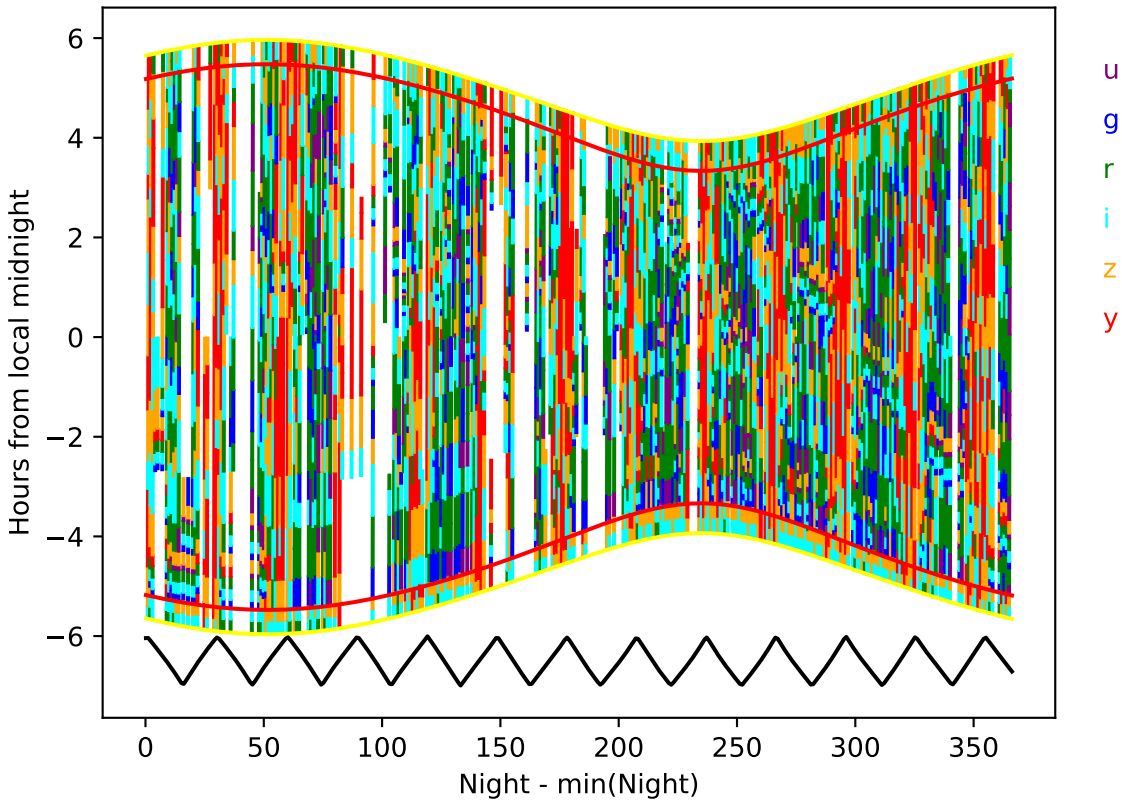
internal_u_expt27_nscale1.2v3.4_10yrs year 1-2: Hourglass
