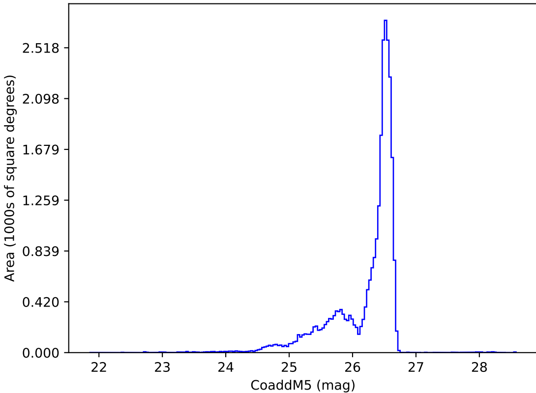
internal_u_expt27_nscale1.2v3.4_10yrs i: CoaddM5
